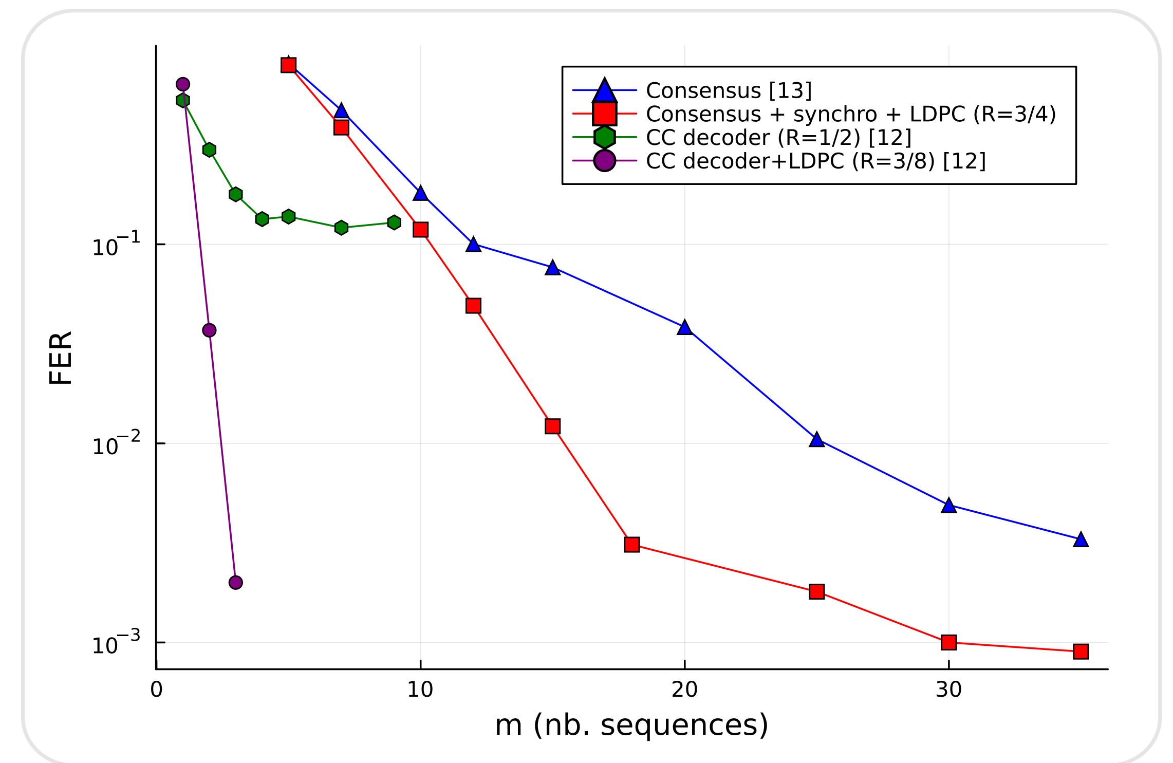
Frame Error Rate by number of sequences for different methods
