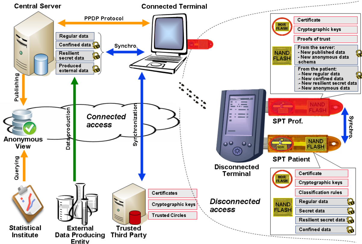
Figure 2: Functional architecture
