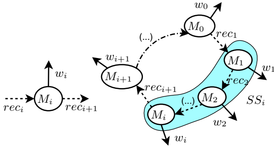
Figure 11: Overview of Milner's scheduler example and the sub-specification SS_i .
