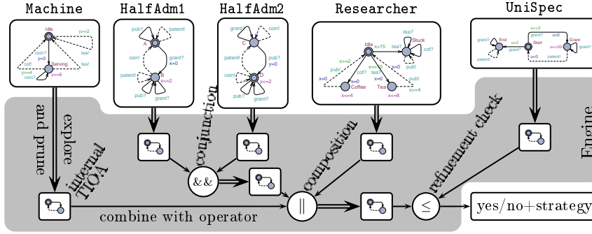
Figure 4: Illustration of the steps performed in a concrete refinement check. The grey box represents the part carried out internally by the verification engine.
