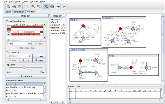
Figure 10: Playing a refinement counter-strategy in the simulator.
