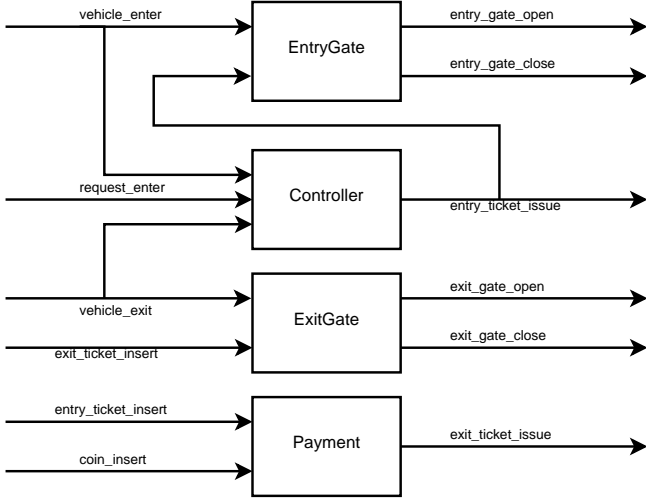
Figure 15: Parking components and communication channels
